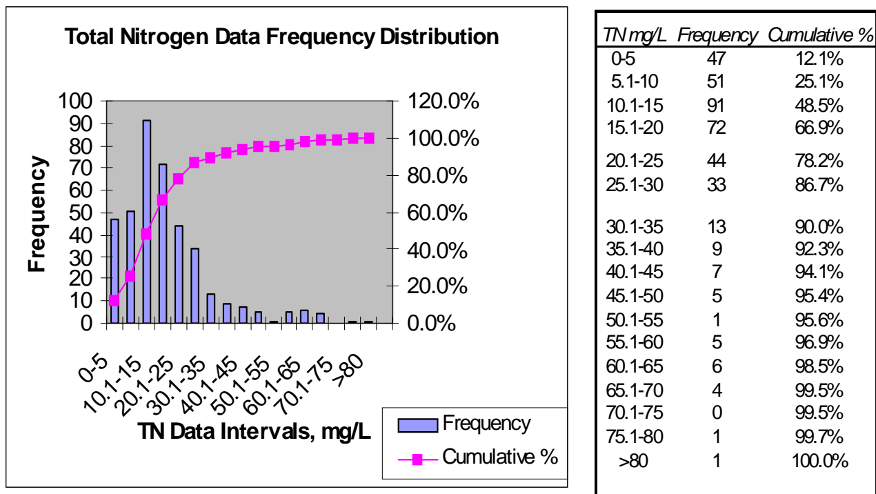
Figure 4. Histogram Showing Data Frequency Distribution for Total Effluent Nitrogen Using Data Shown in Figure 3. Note that 67% of All Samples Meet TN < 20 mg/L Total Effluent Nitrogen, But 33% show TN > 20 mg/L.
